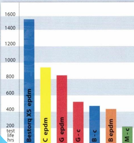
BELT LIFE OF ALL MAJOR BRANDS
