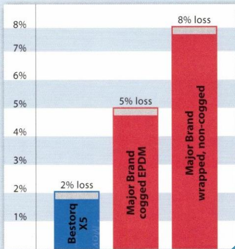
ENERGY LOSS OF V-BELTS FLEXING AROUND PULLEYS
